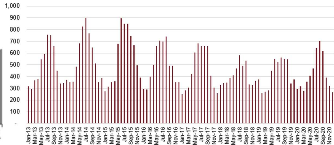
Figure 3. Crude oil used at power stations in Saudi Arabia thousand barrels per day
